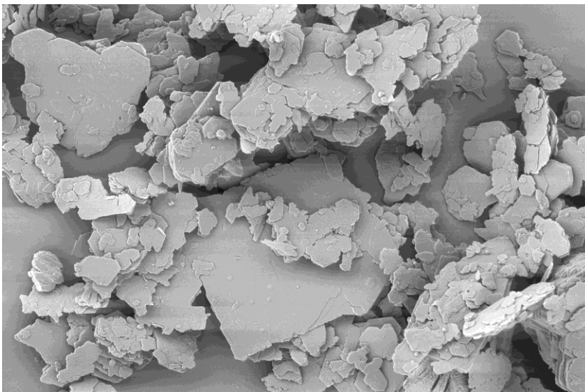
SEM picture shows a typical particle shape which is valid for all our special carbons. The picture above was taken from a larger particle size D 50 10 \mu m.
